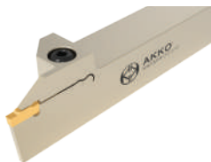
ADKT-RD-R/L-1616-2-T17 ADKT-RD-R/L-2020-2-T17 ADKT-RD-R/L-2525-2-T17 ADKT-RD-R/L-1616-3-T20 ADKT-RD-R/L-2020-3-T25 ADKT-RD-R/L-2525-3-T25 ADKT-RD-R/L-2020-4-T30 ADKT-RD-R/L-2525-4-T30
